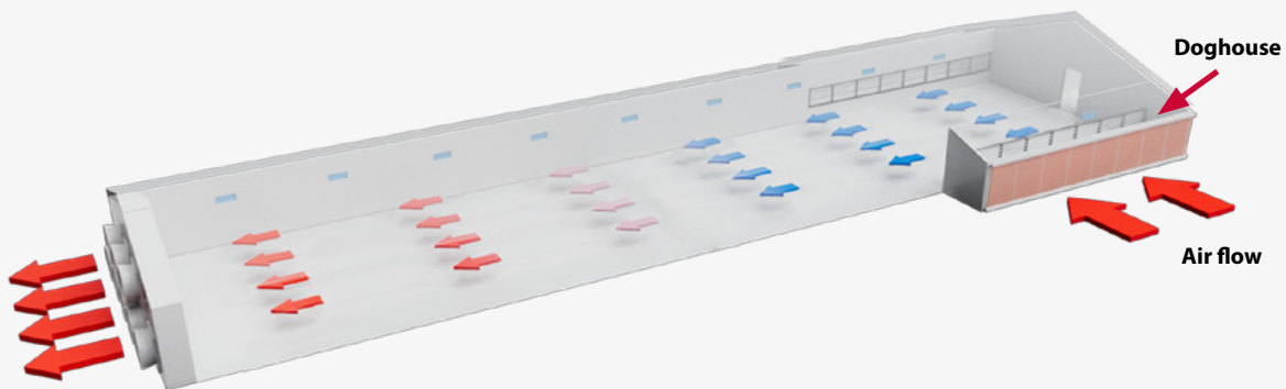
Figure 6.18 Air flow in a tunnel-ventilated house.
