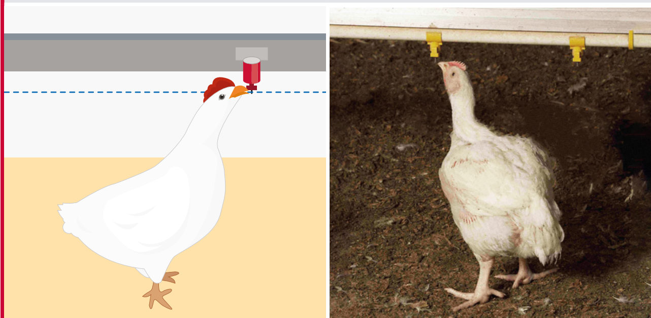
Figure 5.5 Correct nipple drinker height after 7 days (bird's back-to-floor angle: 75–85°).
